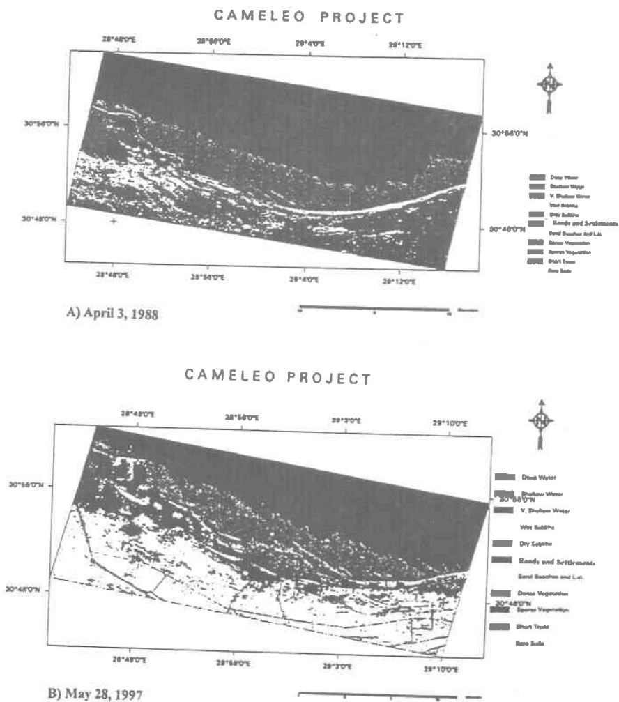
Fig. 2. Unsupervised classified SPOT images of study area.
