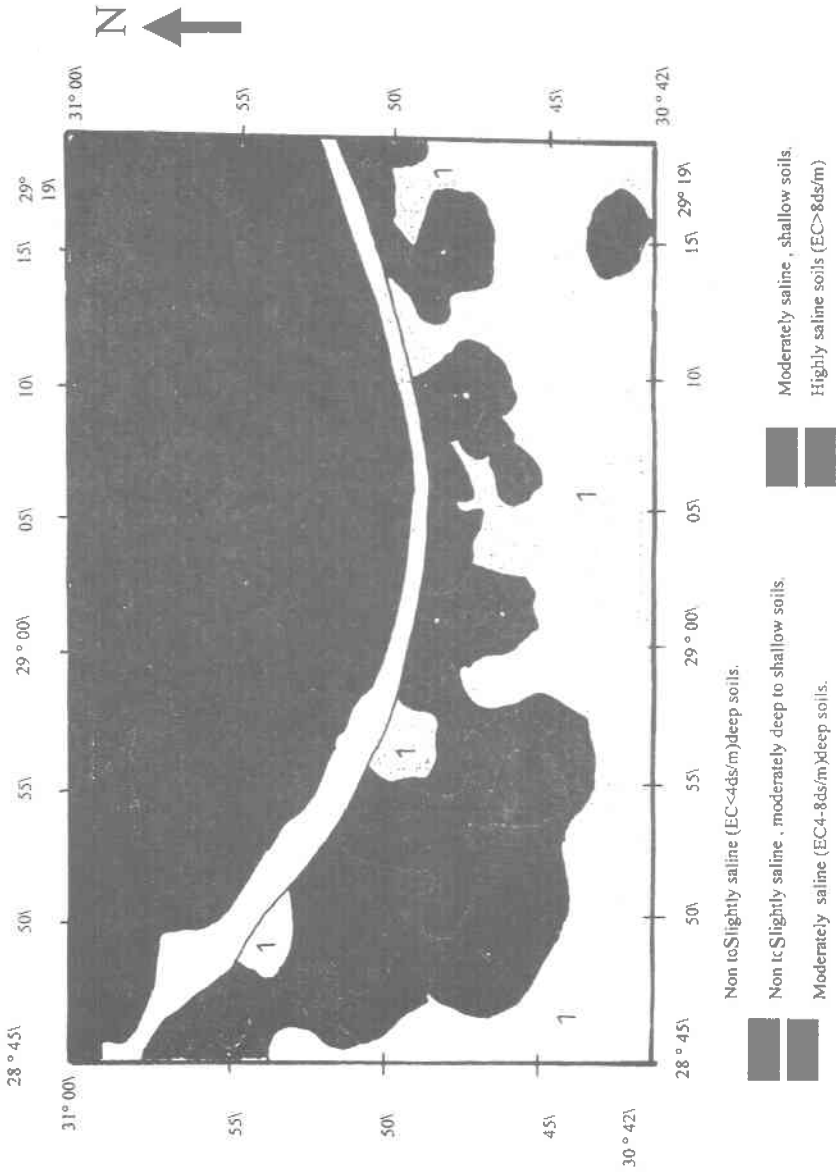
Fig. 3. Soil conditions map of a part of the north western coast, based on FFC of SPOT-XS < 1997.
