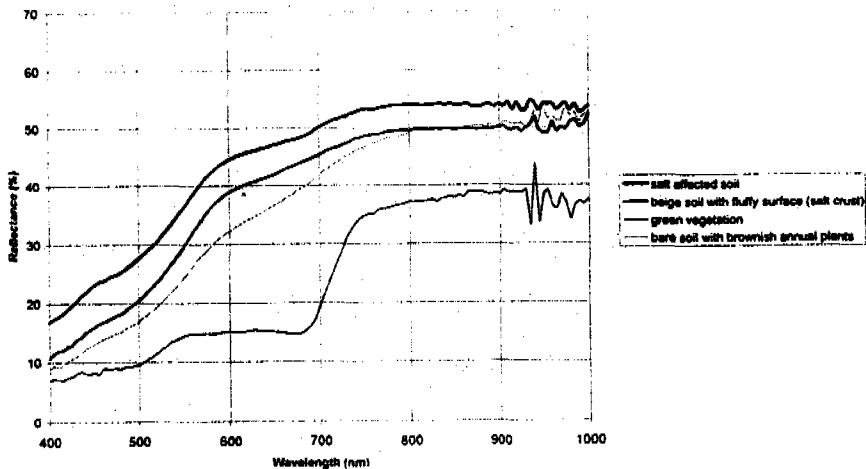
Fig. 5. Field radiometric measurements of the salt affected soils (site No 9).
